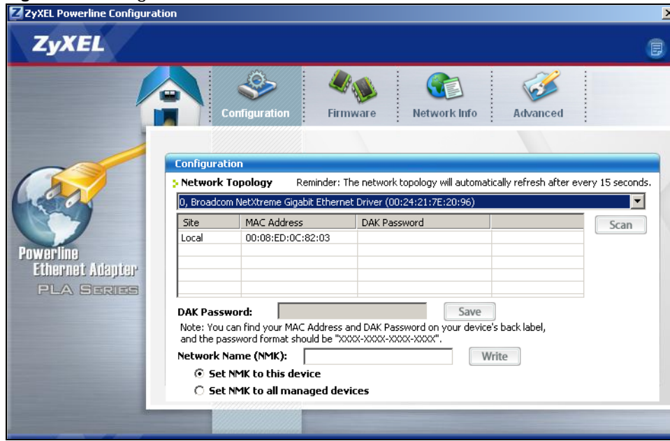
Figure 13 Configuration Screen
