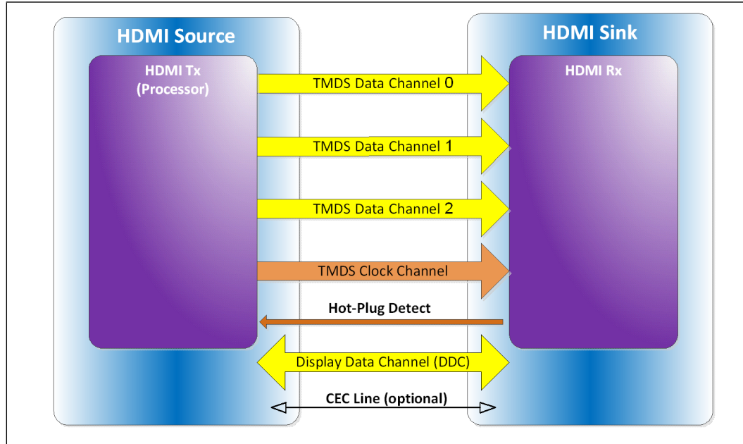
Figure 2-8. HDMI* Overview
