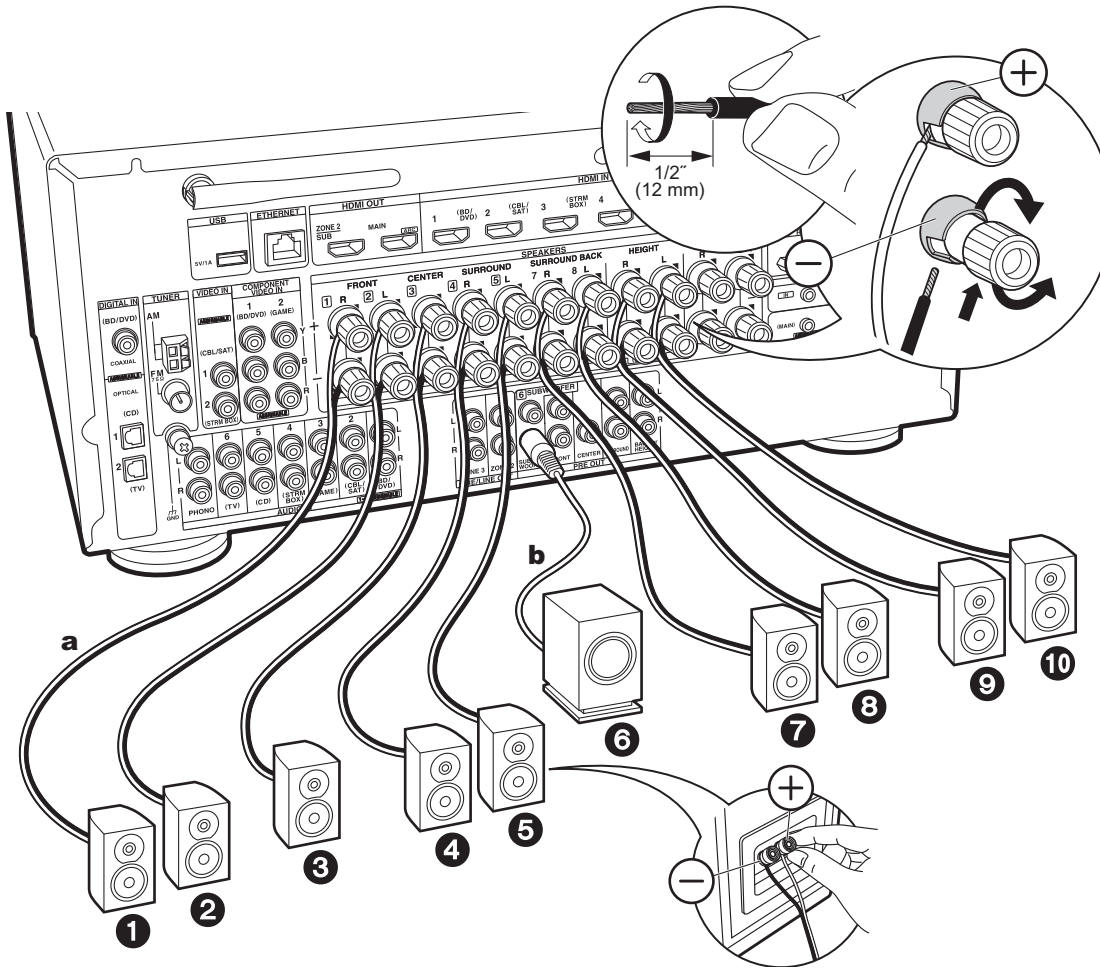
a Speaker cable, b Subwoofer cable
