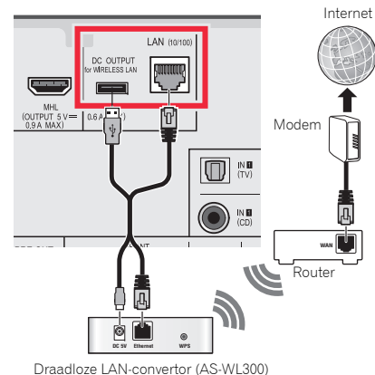
Draadloze LAN-converter (AS-WL300)
