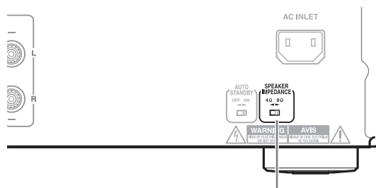
SPEAKER IMPEDANCE selector
