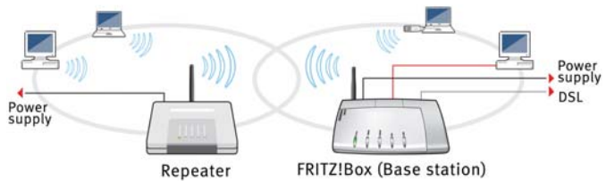
WDS: Expanding the WLAN range using a repeater
